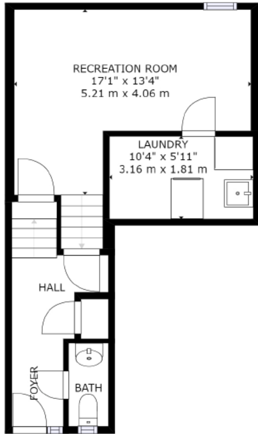
BASEMENT
